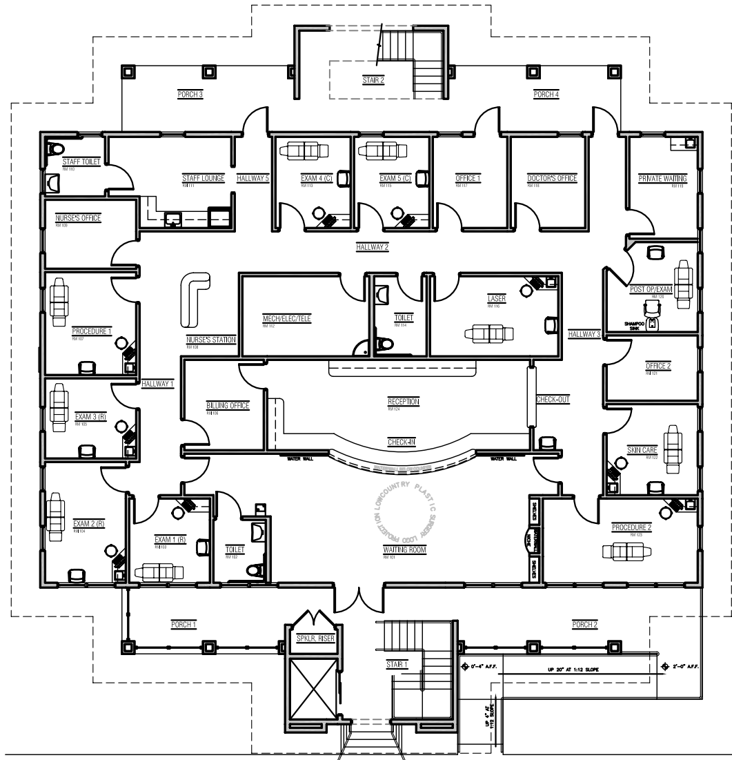
Building 2 - first floor
